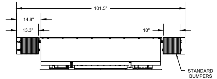
FRONT ELEVATION
