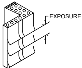
WEAR PLEATS DETAIL
