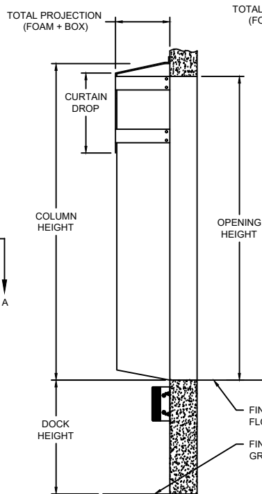
SECTION B-B
