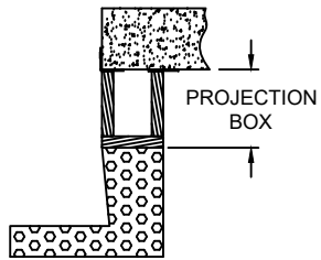
PROJECTION BOX DETAIL
