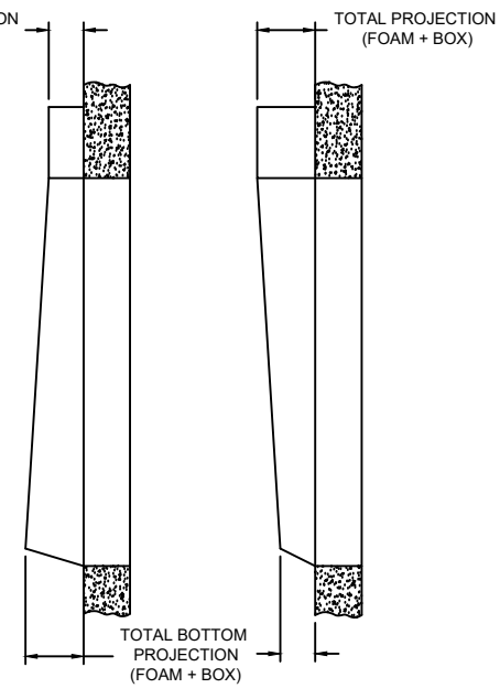
SECTION B-B TAPERED UP
