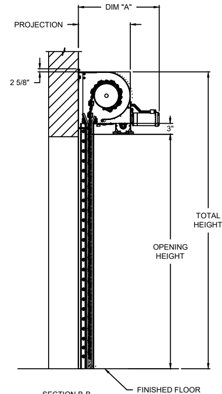
SECTION B-B
