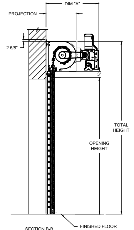
SECTION B-B
