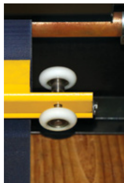
Wind strut with roller windlocks
