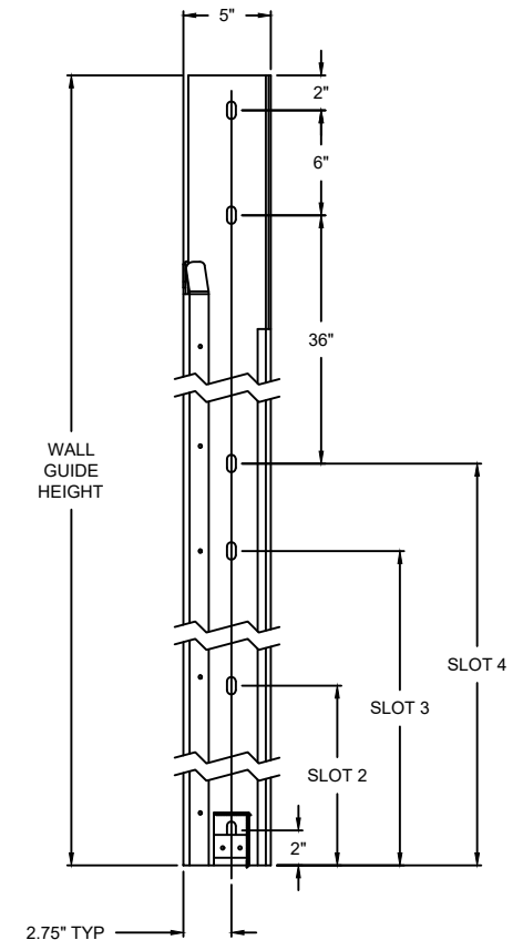
NO SPLICE JAMB DETAIL SHOWING 6 SLOTS
